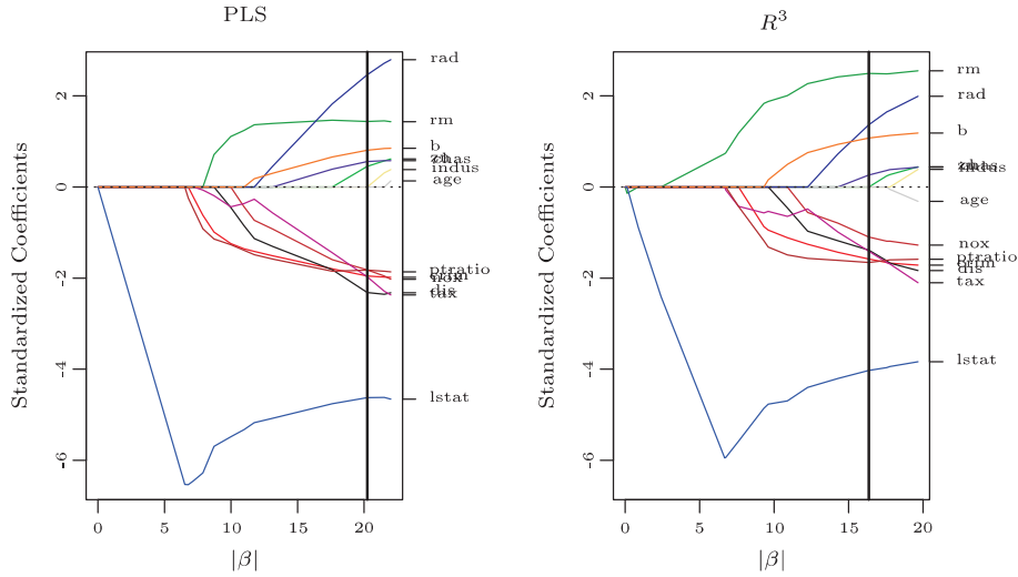
Figure 3.3. The solution paths for the Boston housing data set. The coefficients are standardized by the corresponding standard errors of the covariates. The vertical black lines indicate the chosen models.
